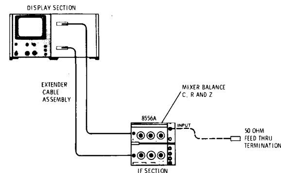
Figure 5-4. Mixer Balance Adjustments Test Setup
