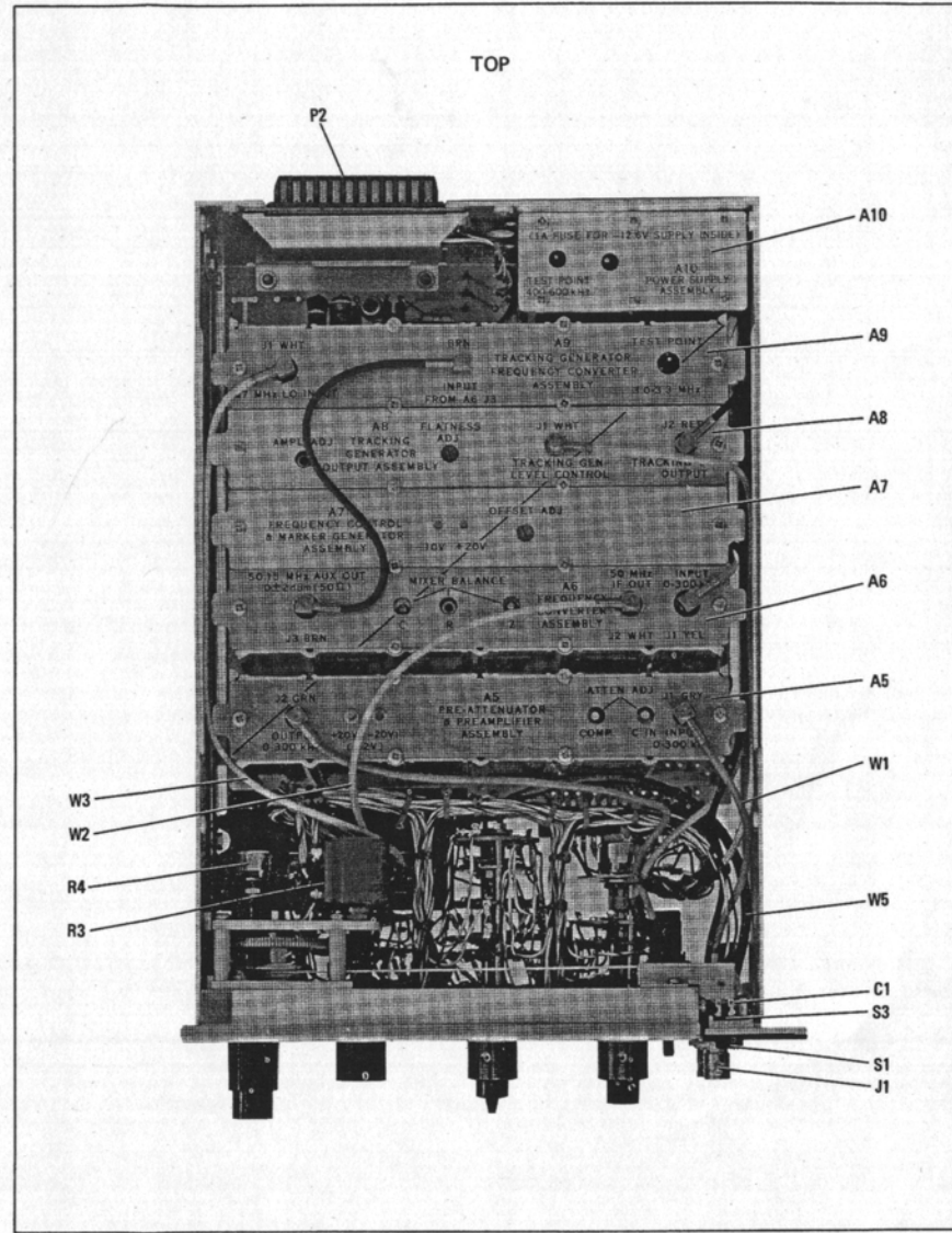
Figure 8-14. Top and Bottom Internal View.
