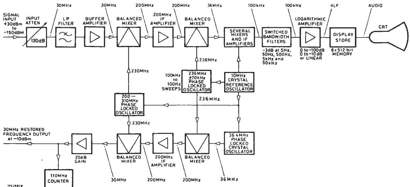
Fig. 3.1 Simplified overall impression of TF 2370
