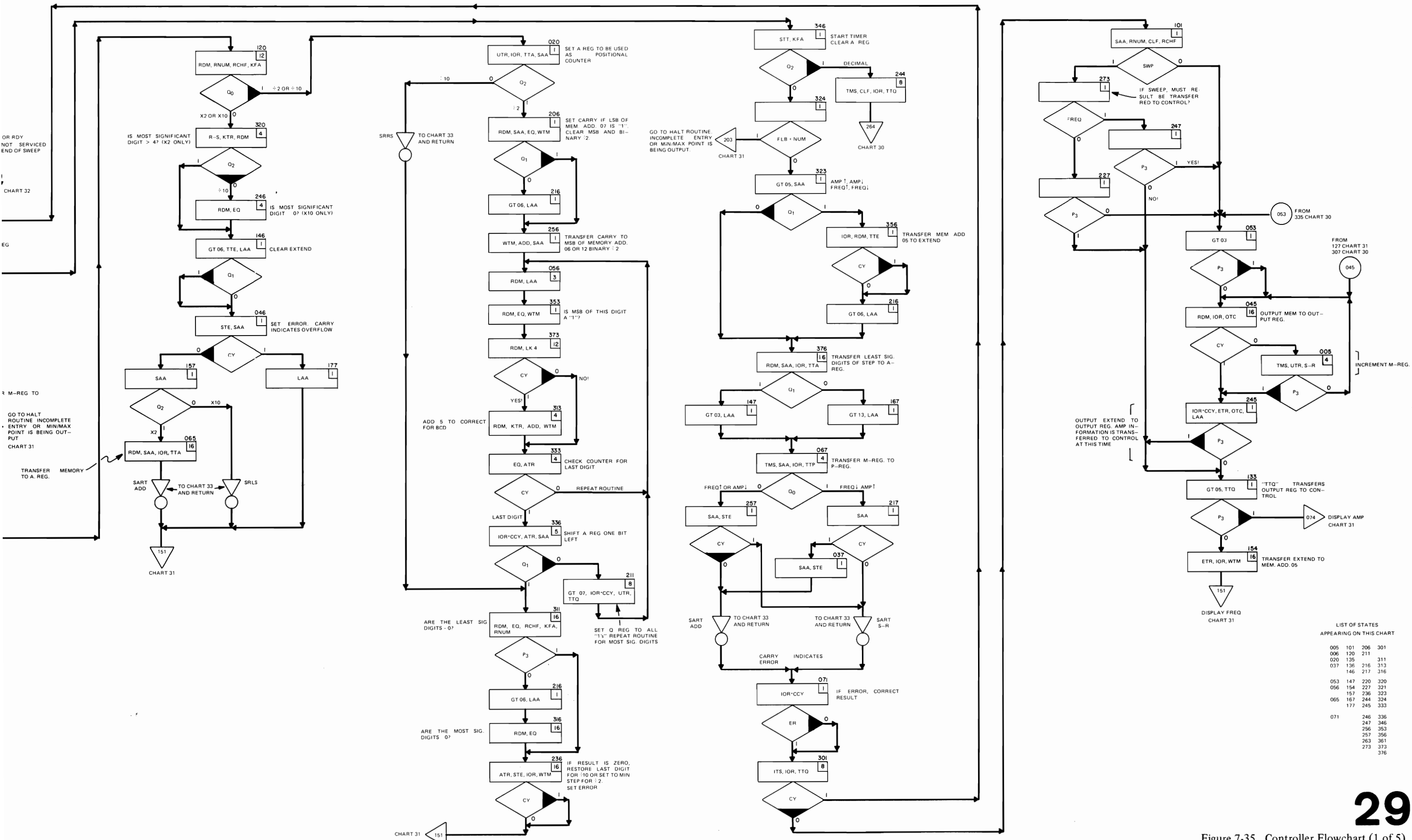
Figure 7-35. Controller Flowchart (1 of 5). 7-105/7-106
