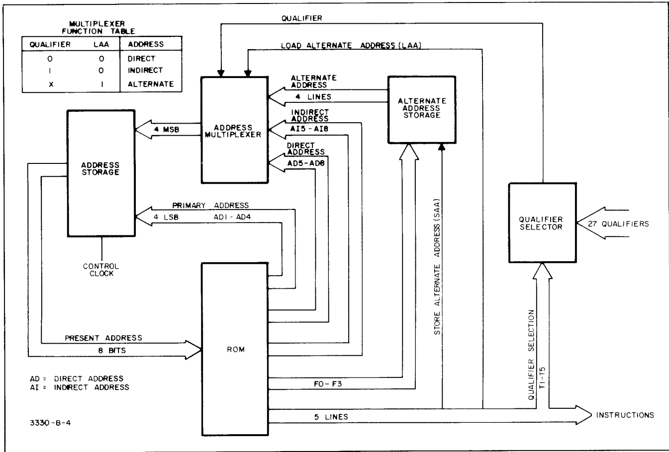
Figure 4-14. Address Selection.
