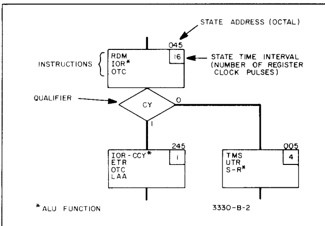
Figure 4-12. Flowchart Example.
