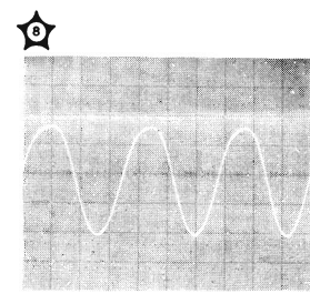
8. MEASUREMENT POINT: XA24 SL1RF OSCILLOSCOPE SETTINGS: VOLTS/DIV .01 TIME/DIV .1 μsec HORIZONTAL MAG X10
