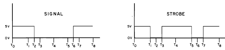
SIGNAL TIMING DIAGRAM Example
