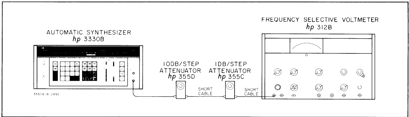
Figure 5-1. Harmonic Distortion.
