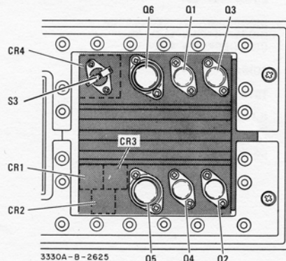
p/o Figure 6-1. Chassis Mounted Components.
