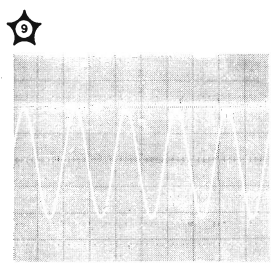
9. MEASUREMENT POINT: XA23 IF OSCILLOSCOPE SETTINGS: VOLTS/DIV .05 TIME/DIV 2 μsec HORIZONTAL MAG X1 dc OFFSET 7.75 V
