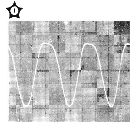
1. MEASUREMENT POINT: XA15 N1RF OSCILLOSCOPE SETTINGS: VOLTS/DIV .01 TIME/DIV .1 μsec HORIZONTAL MAG X10
