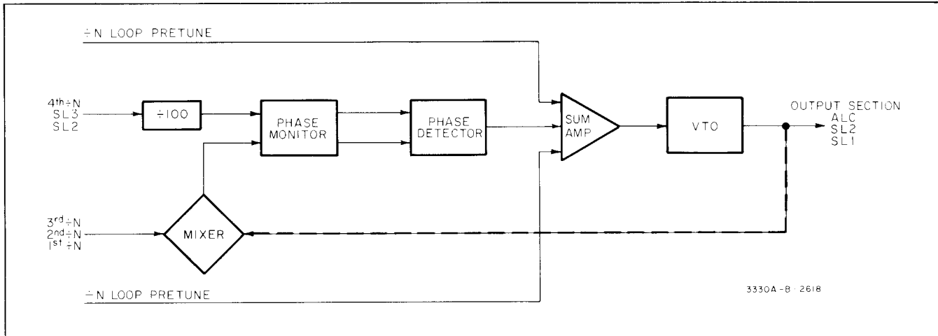
Figure 4-5. SL Loop.
