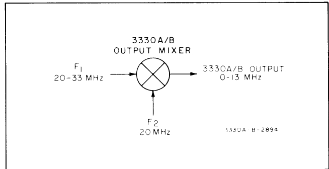
Figure 5-3. 3330 Output Section.
