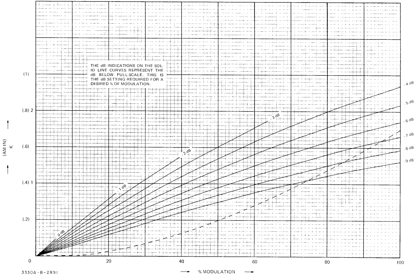
Figure 3-1. AM IN.
