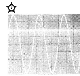
7. MEASUREMENT POINT: XA24 N1SL1RF OSCILLOSCOPE SETTINGS: VOLTS/DIV .005 TIME/DIV .1 μsec HORIZONTAL MAG X10
