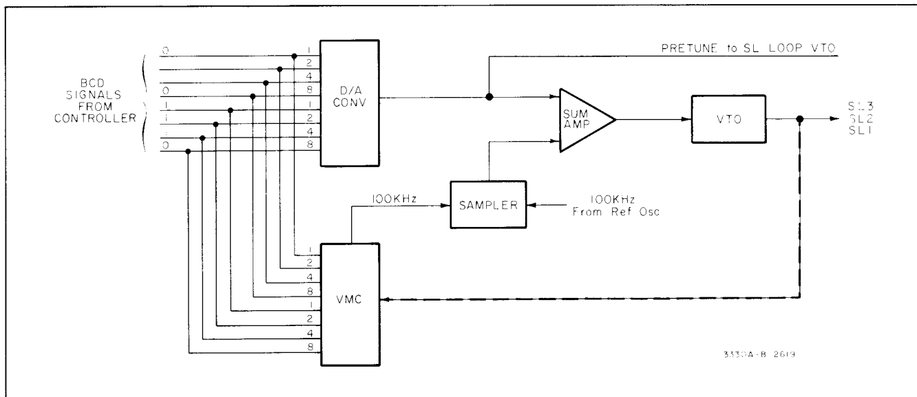
Figure 4-4. ÷ Loop.
