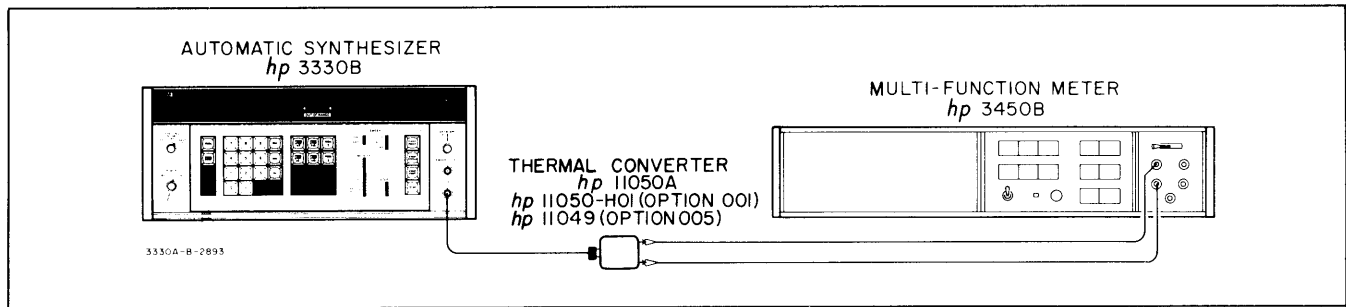
Figure 5-5. Frequency Response.
