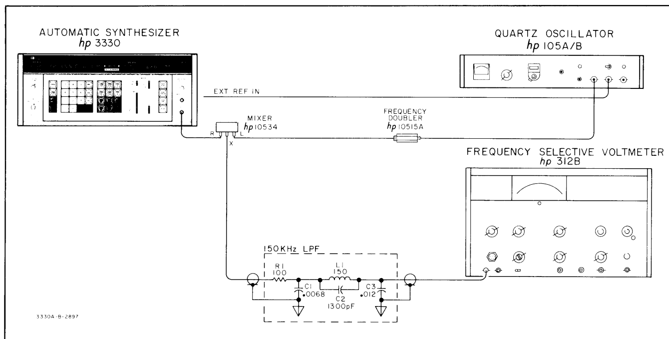
Figure 5-4. Spurious.
