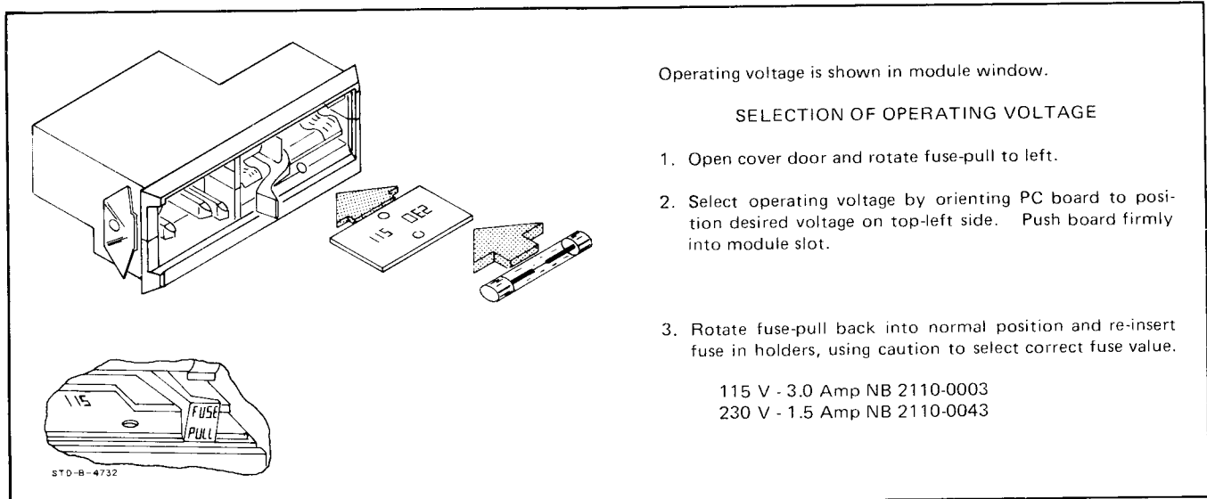
Figure 2-1. Voltage Selection.
