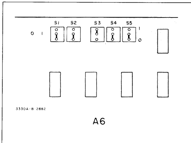
Figure 3-3. Addressing Jumpers.
