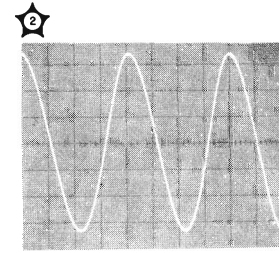
2. MEASUREMENT POINT: XA13 N2RF, XA11 N3RF OSCILLOSCOPE SETTINGS: VOLTS/DIV .01 TIME/DIV .1 μsec dc OFFSET 0.62 V HORIZONTAL MAG X10
