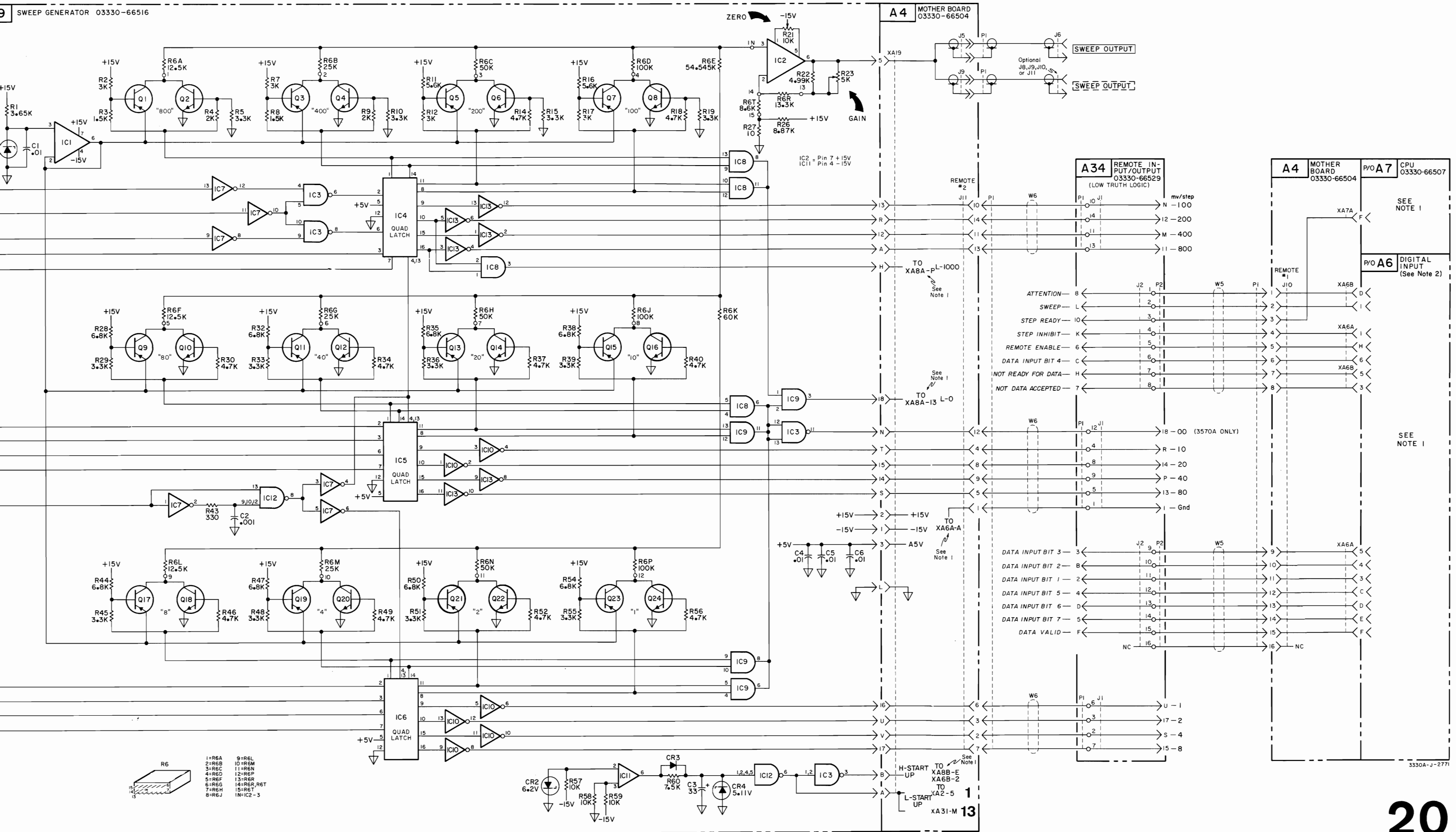
Figure 7-26. Sweep Generator A19, Remote Input/Output A34. 7-63/7-64
