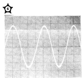
6. MEASUREMENT POINT: XA21 N2SL2RF OSCILLOSCOPE SETTINGS: VOLTS/DIV .005 TIME/DIV .1 μsec HORIZONTAL MAG X10
