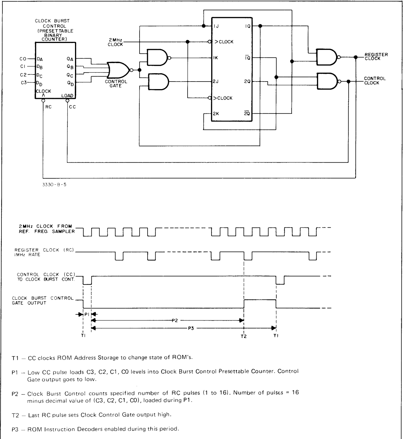
Figure 4-15. Clock Generator.
