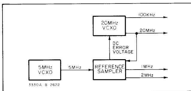
Figure 4-2. Reference Oscillator.
