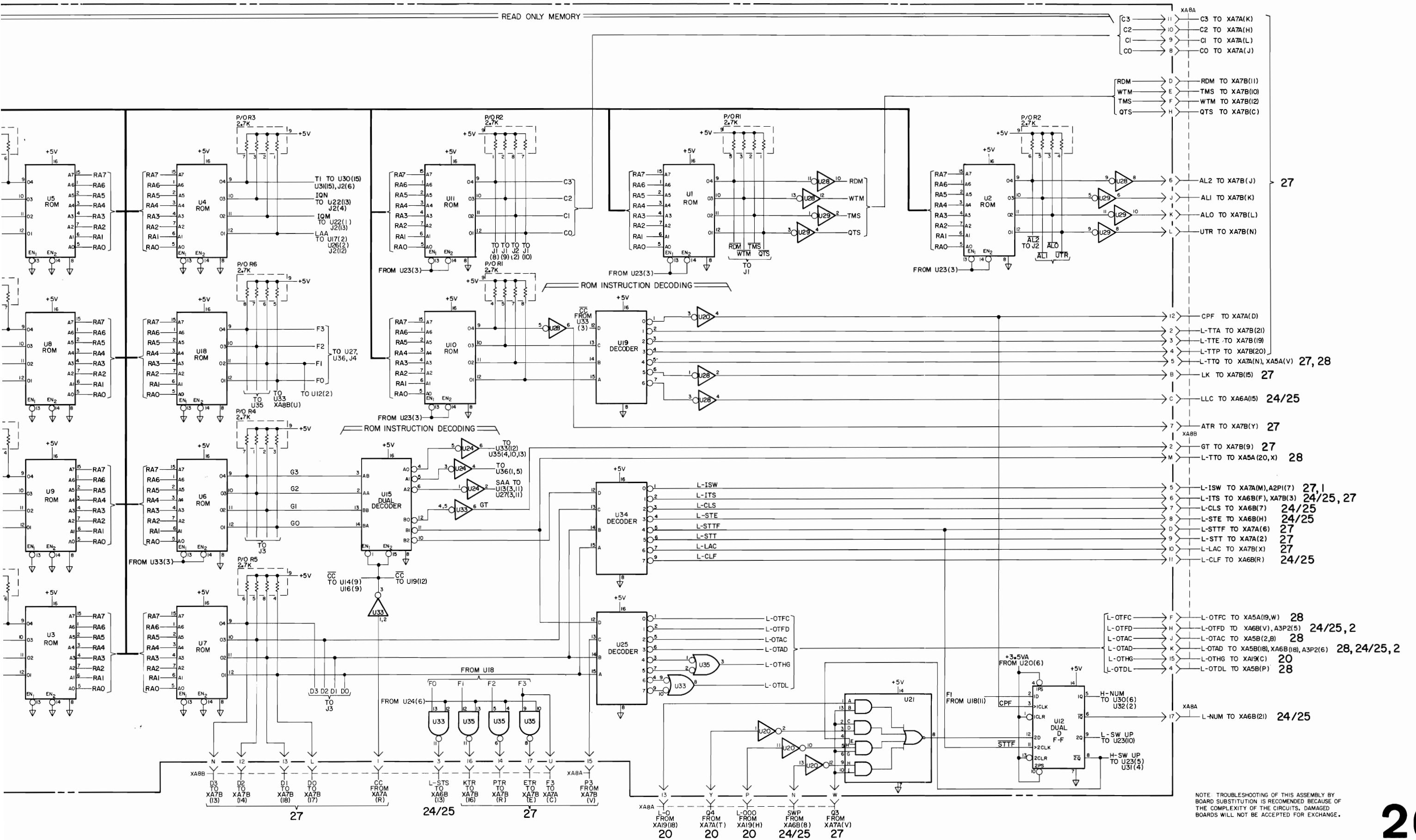
Figure 7-32. Control Assembly, A8.
