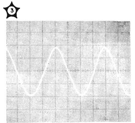
3. MEASUREMENT POINT: XA9 N4RF OSCILLOSCOPE SETTINGS: VOLTS/DIV .01 TIME/DIV .1 μsec dc OFFSET 0.7 V HORIZONTAL MAG X10
