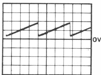
EACH DIV. = 2V, 10 \mu S PIN 7 of U4
