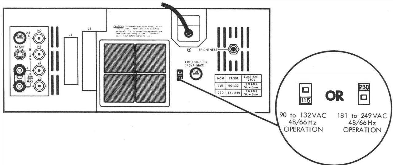
Figure 2-5. Line Voltage Settings
