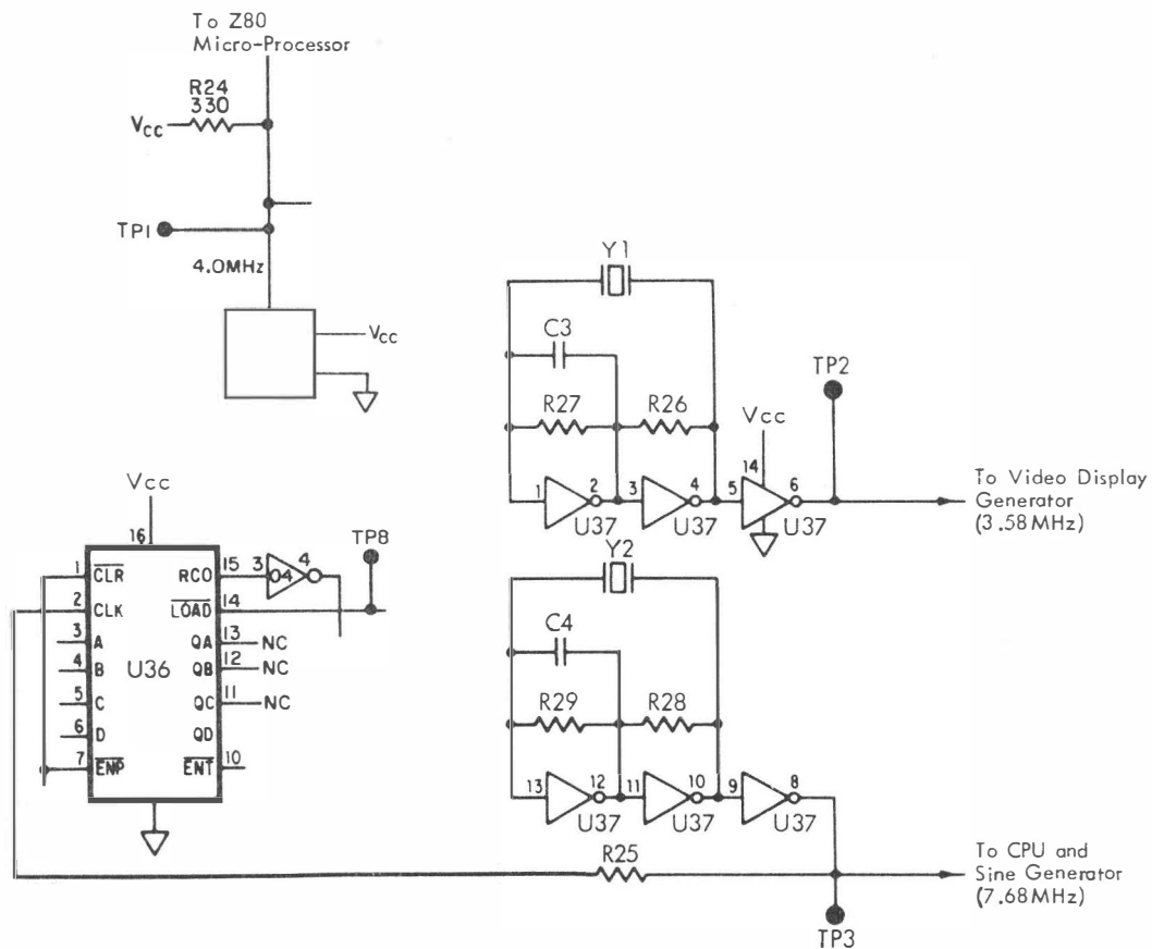
Figure 3-14. Clock Signals
