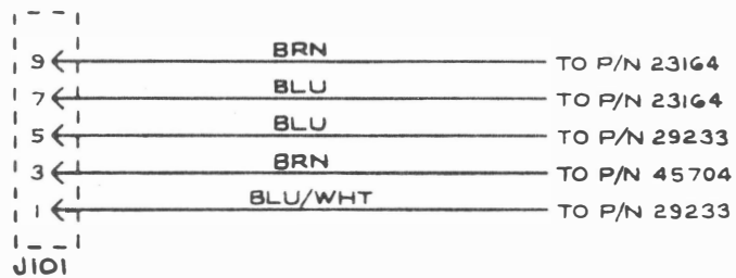
Figure 5-11. Back Panel-to-Power Supply Cable Assembly (P/N 47115)
