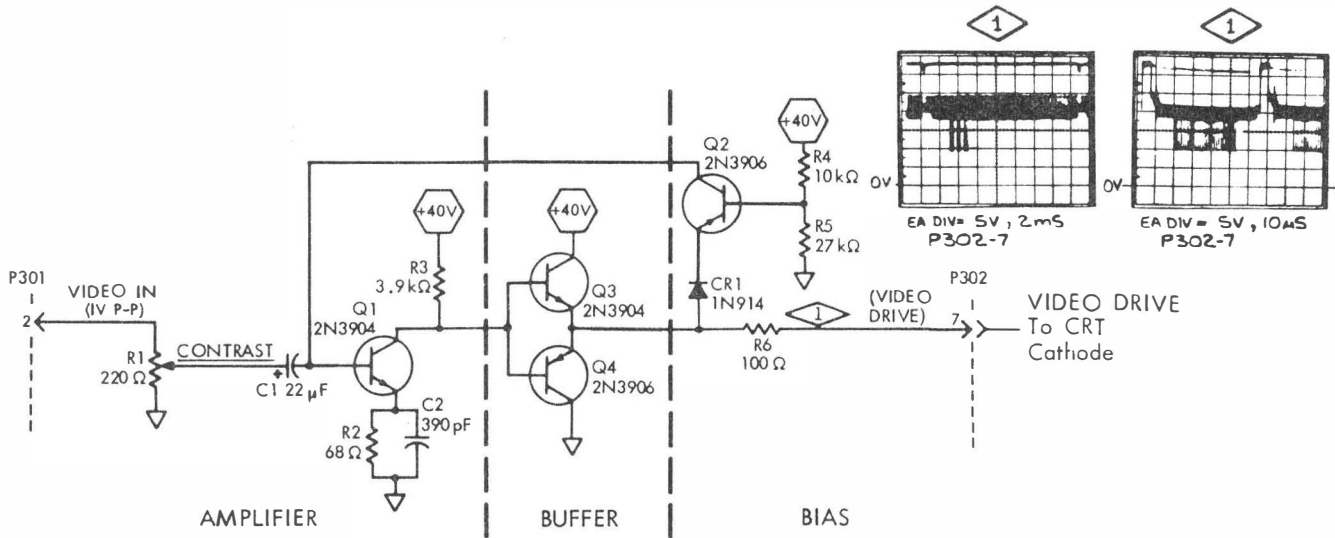
Figure 3-17. Video Amplifier
