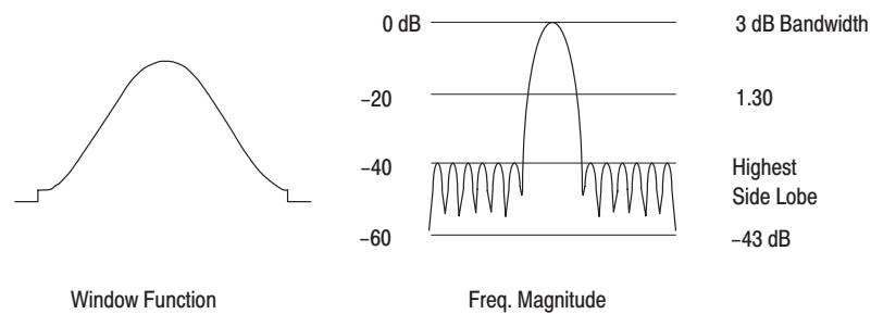
Figure F-10: Hamming Window and Frequency Characteristic
