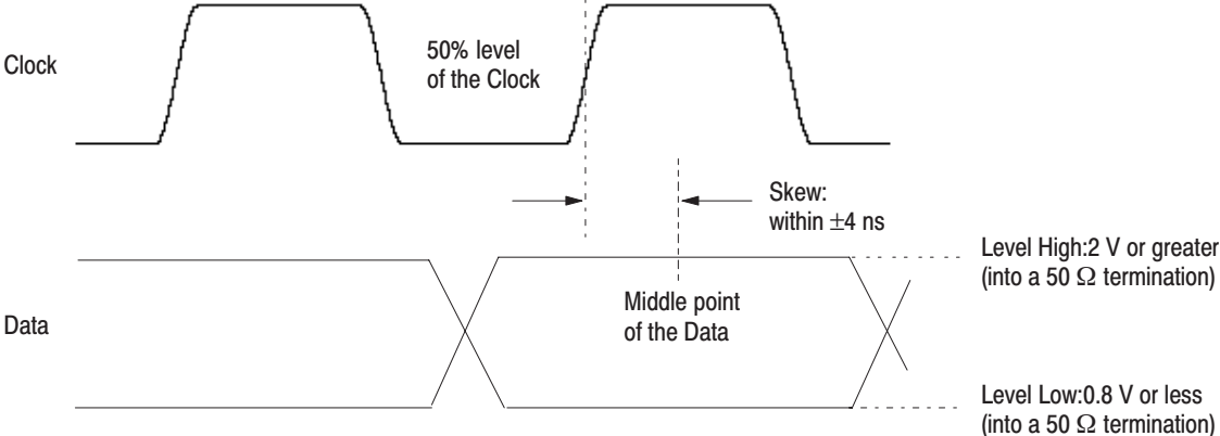
Figure A-14: Output Waveform
