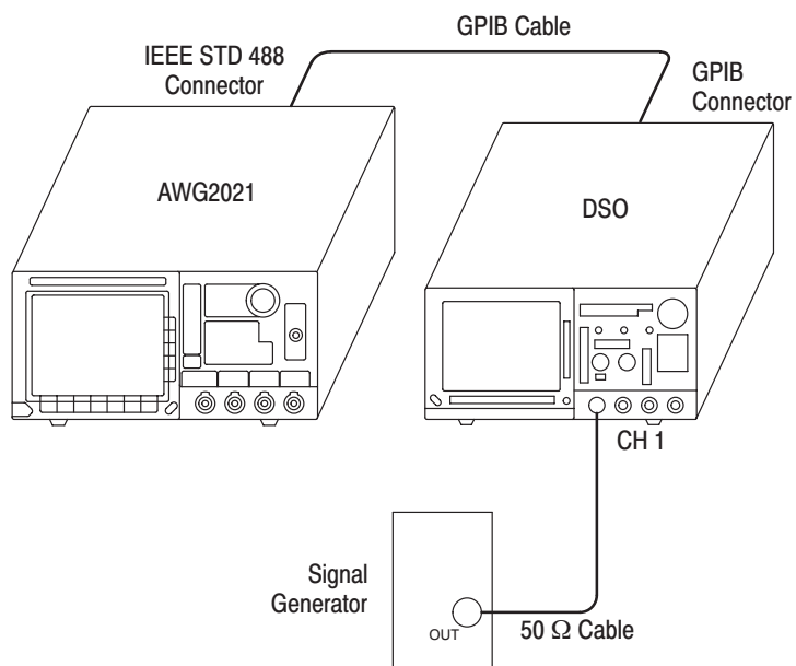
Figure 2 -62: Connections for Example 5
